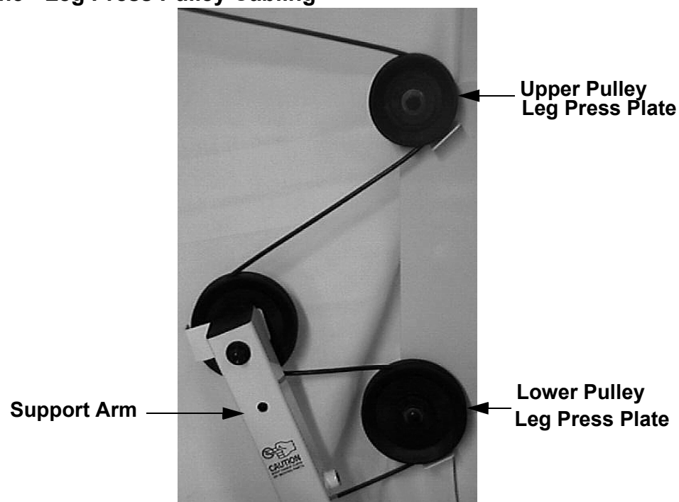
Diagram 4.5 - Leg Press Pulley Cabling
